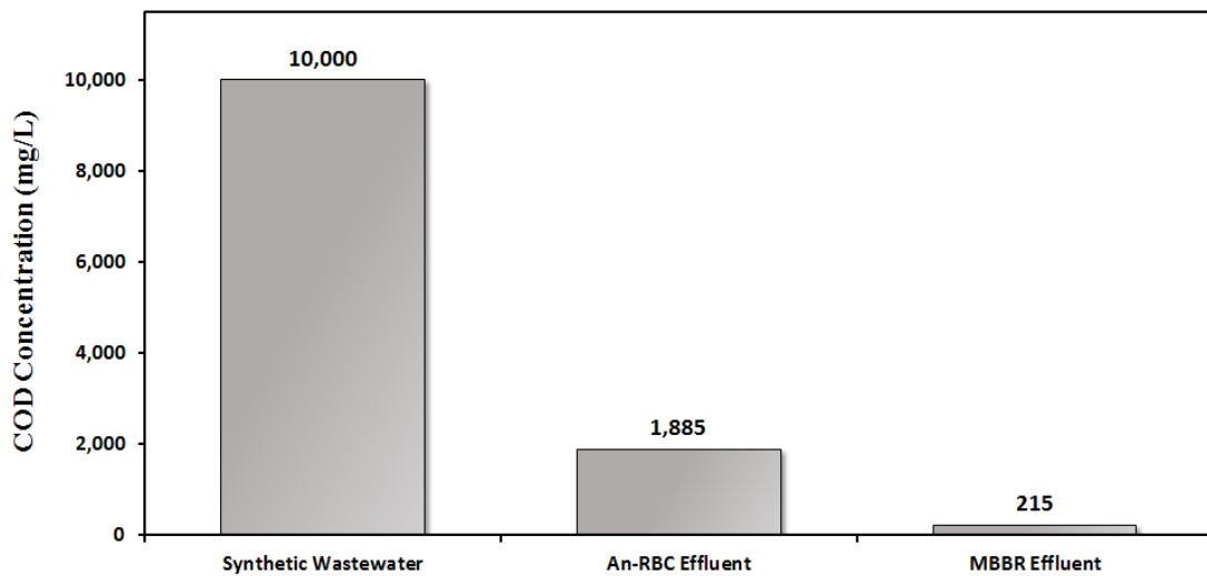
Figure 4-10. COD concentrations under selected optimal operational conditions
