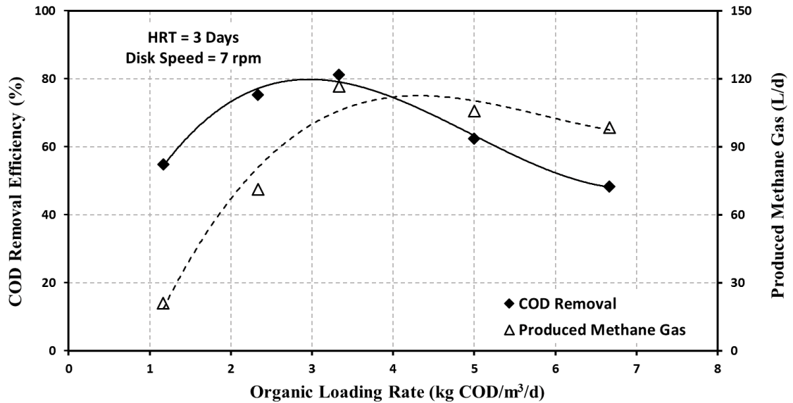
Figure 4-3. The effect of OLR on COD removal efficiency and produced methane in the anaerobic reactor
