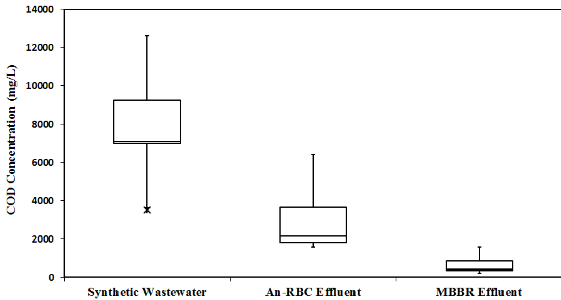
Figure 4-9. COD concentrations from all conducted experiments. The box illustrates the 25th percentile, median, and 75th percentile. The top and bottom whiskers represent the highest and lowest values
