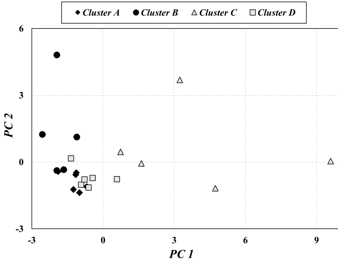
Figure 6-3. PCA scores from samples from different clusters
